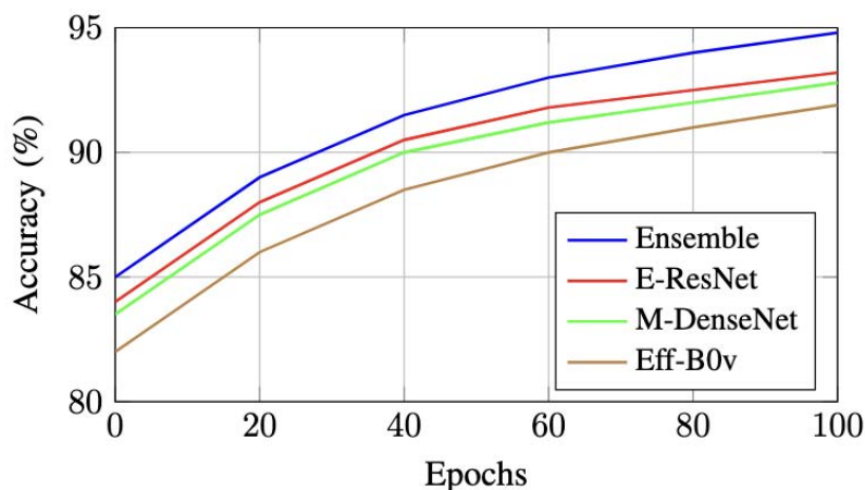
Fig.1: Training Accuracy Progression Across Different Architectures
